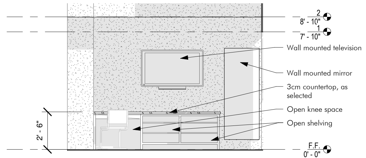
2 1 - c SCALE 1/4" = 1'-0"
