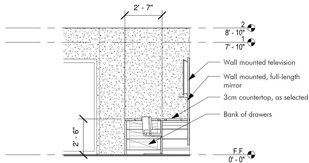
3 1 - b SCALE 1/4" = 1'-0"
