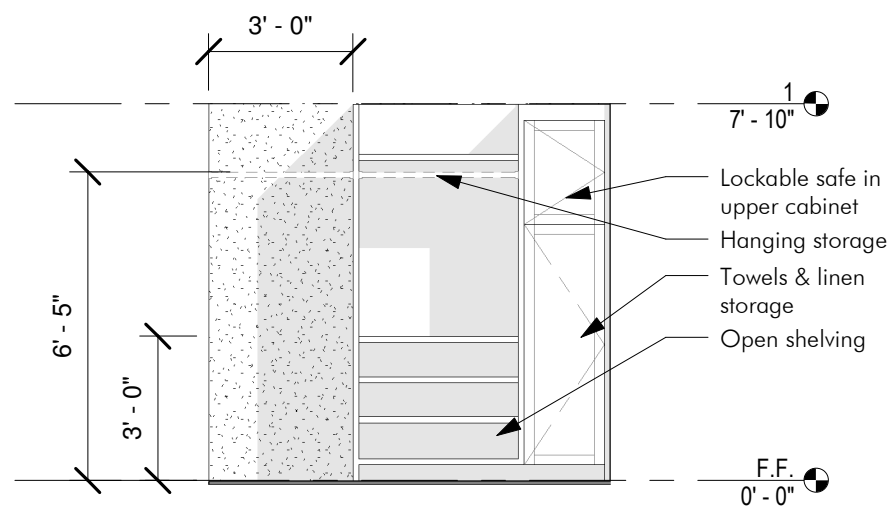
4 Elevation 1 - c SCALE 1/4" = 1'-0"
